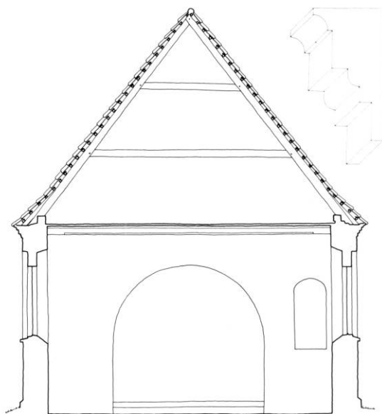
Fig. 5. Tværnit set mod øst 1:150. Målt af John Bennetzen 1989, tegnet af KdeFL 1993. Snit i gesims 1:20, KdeFL 1993. - Cross-section of the nave looking east and section of the cornice of the building.
